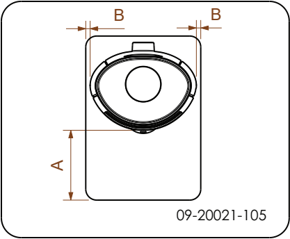
Minimum dimensions of fireproof floor plate
